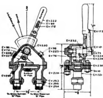
Figs. 2567-2568. 3/4-Inch Straight-Air Brake Valve.
